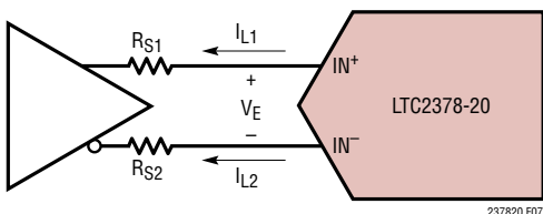
Figure 7. Source Impedances of a Driver and Input Leakage Currents of the LTC2378-20
