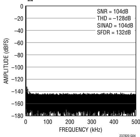
128k Point FFT f_S = 1\text{Mps} , f_{IN} = 2\text{kHz}
